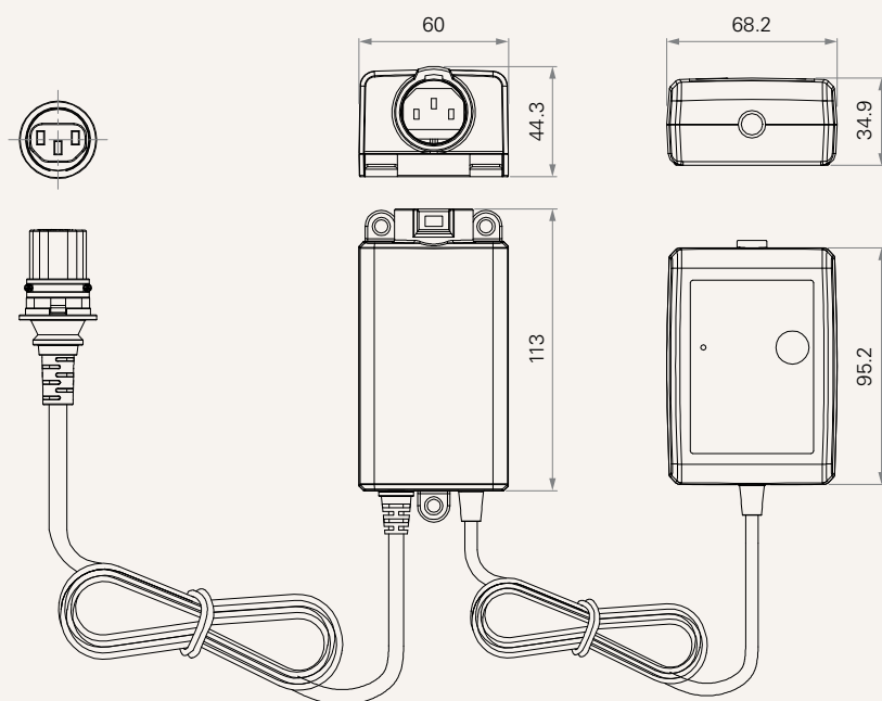
AC cable connect to control box
